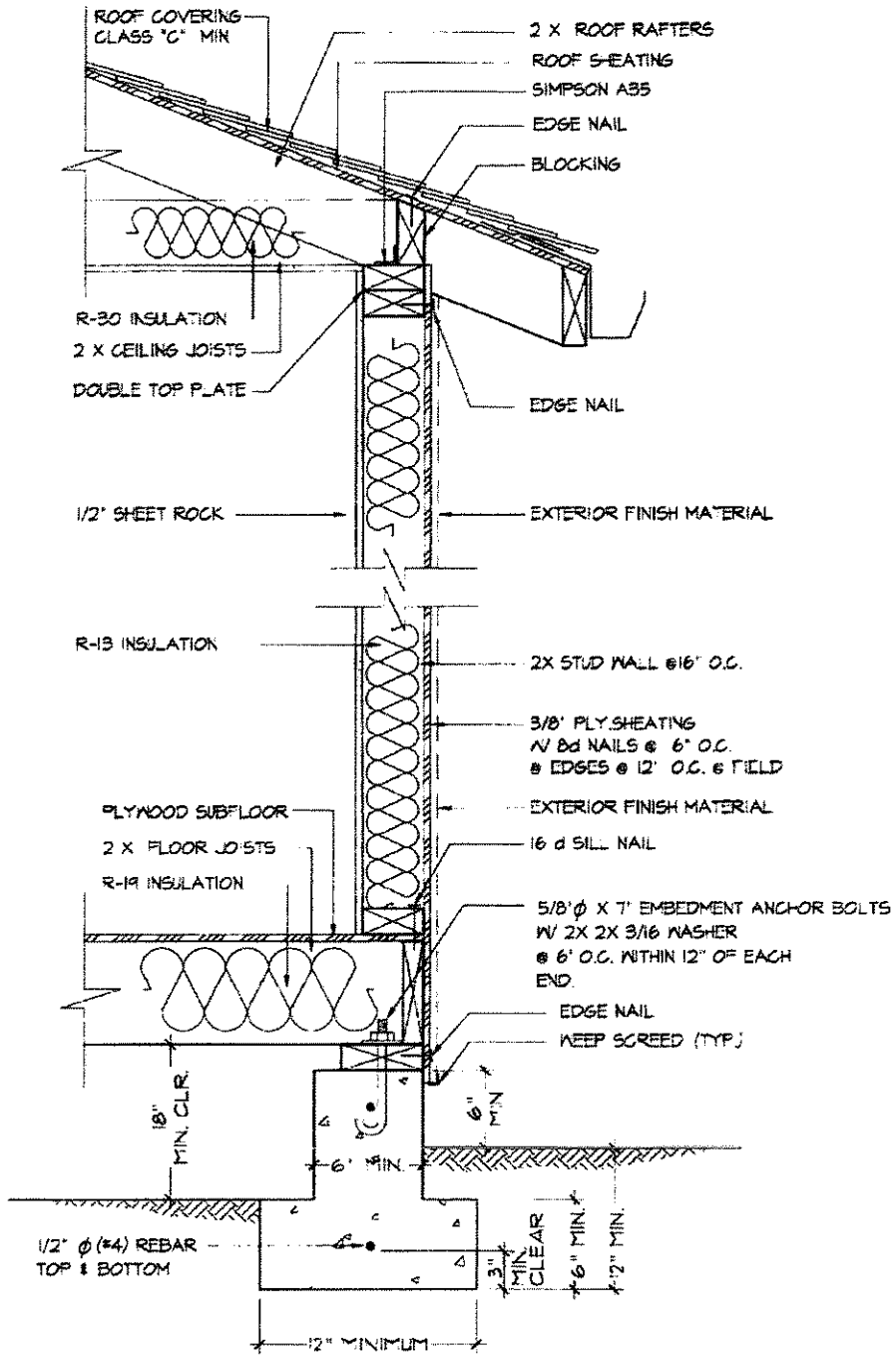
EXTERIOR WALL CROSS SECTION
