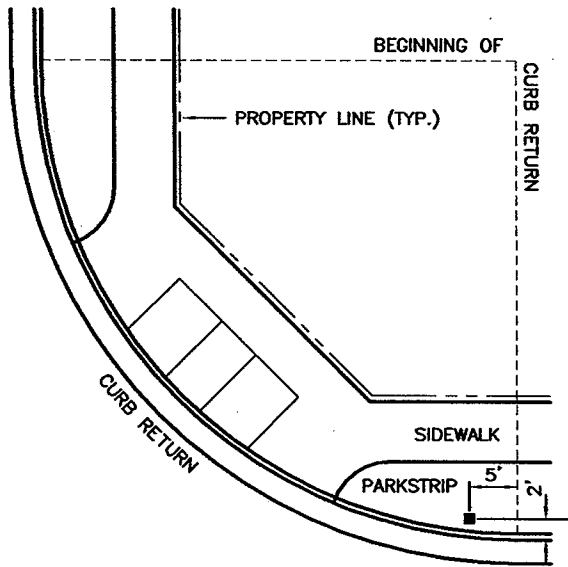
SIDEWALK WITH PARKSTRIP
