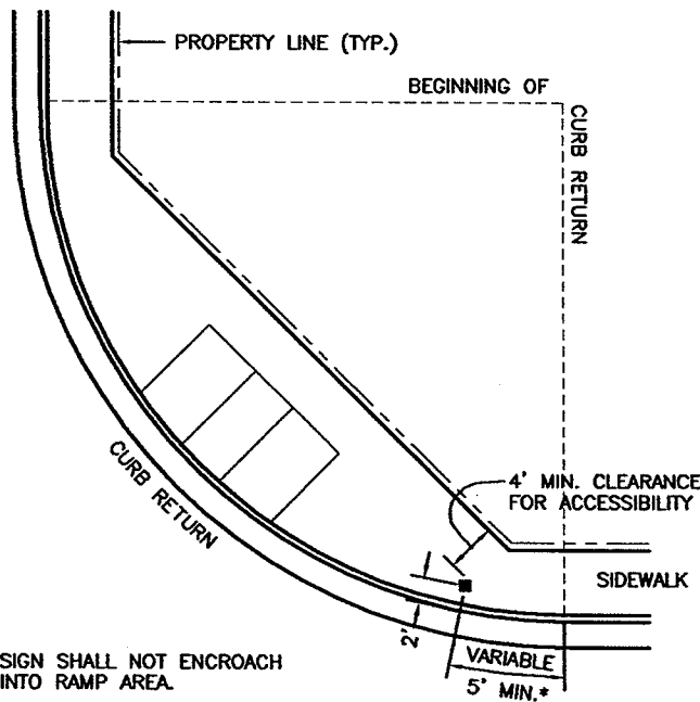
SIDEWALK ADJACENT TO CURB
