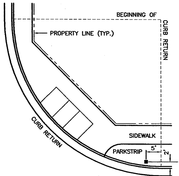
SIDEWALK TRANSITION FROM ADJACENT TO NOT ADJACENT TO CURB
